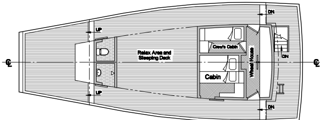
TOP DECK
