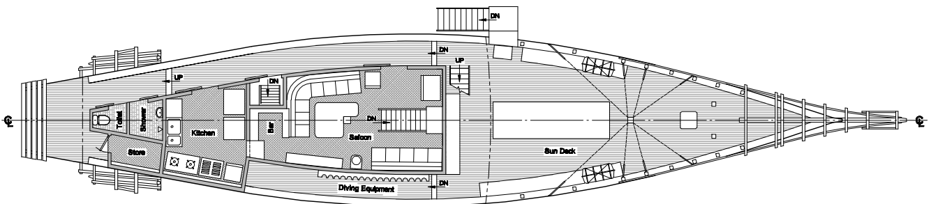
MAIN DECK
