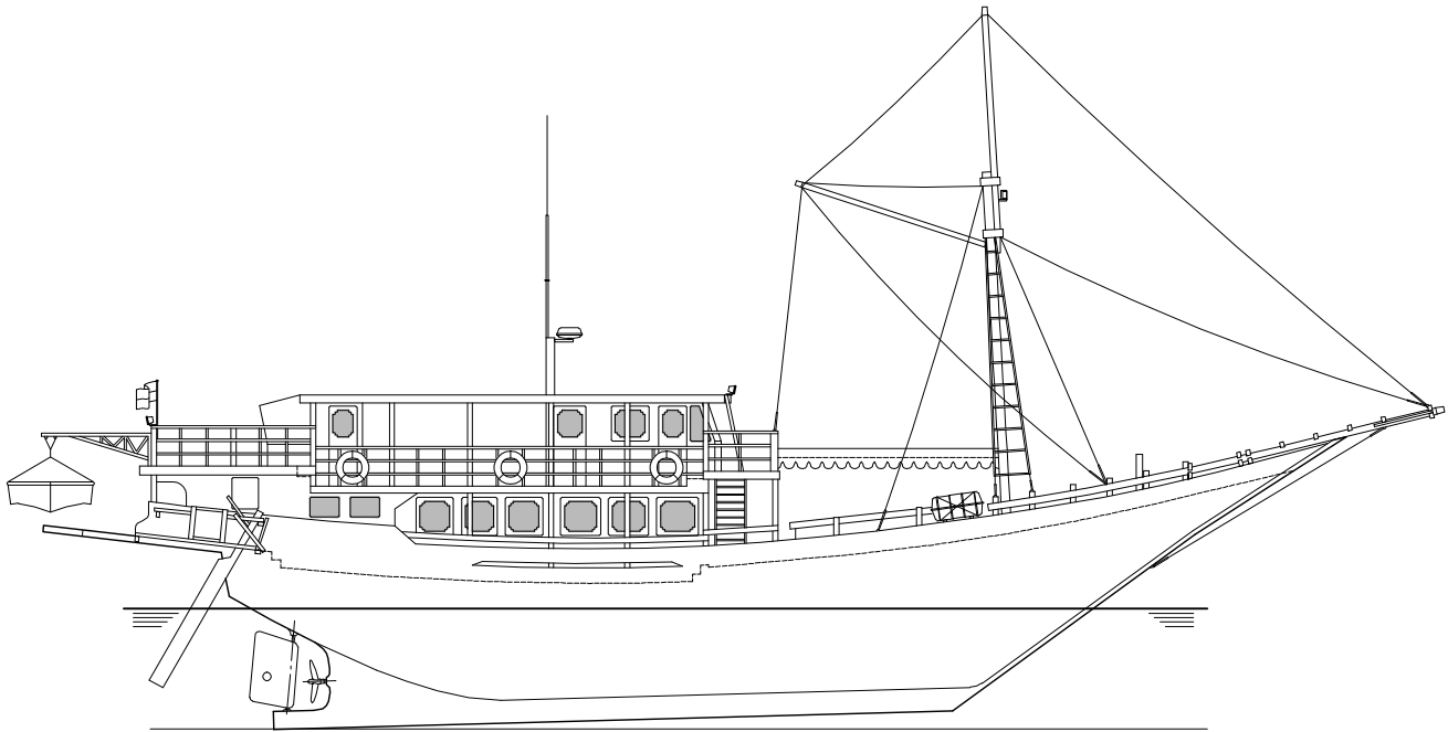
SIDE VIEW
